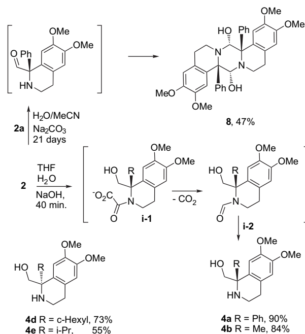
Scheme 2. Hydrolysis of nitrogen substituent in 2 leading to formation of \beta -amino alcohols via intramolecular Canizzaro reaction.
