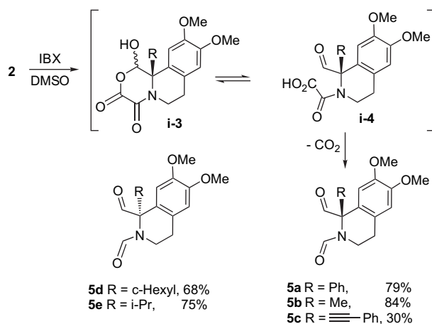
Scheme 3. Oxidation of 2 leading to N -formyl aldehydes.
