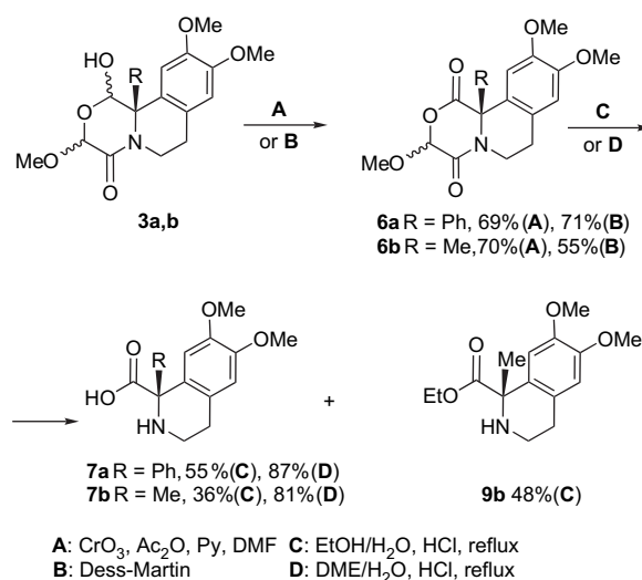
Scheme 4. Synthesis of (+)-6,7-dimethoxy-salsoline-1-carboxylic acid 7b and its 1-phenyl analogue 7a .
