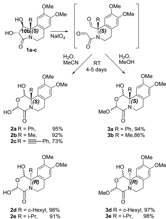
Scheme 1. Glycolic cleavage of 1,2-dihydroxy-hexahydro-pyrrolo-isoquinolines 1a–e .
